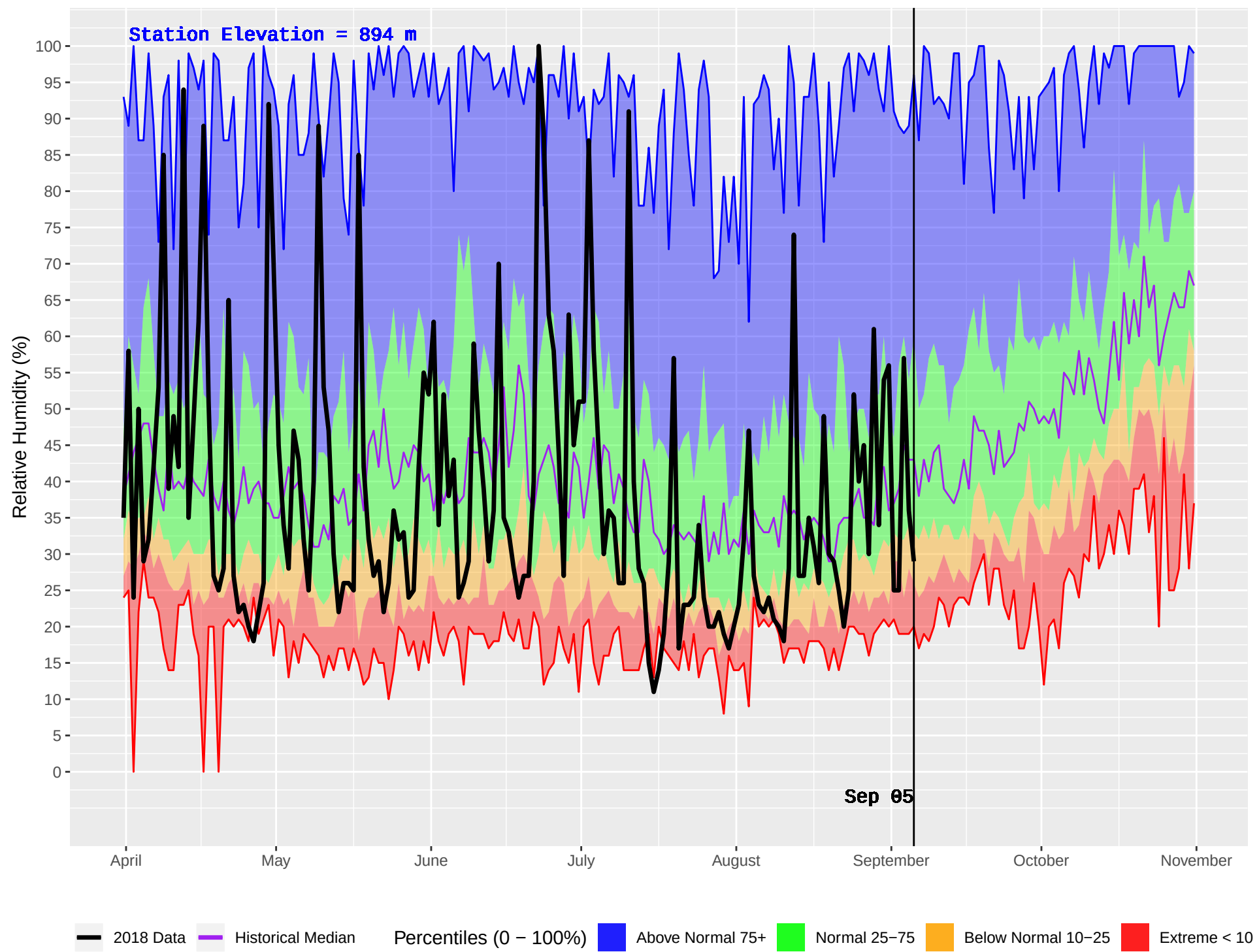
TOBY HUB (417) : Historical (1986–2016) and Current (2018) Daily Relative Humidity
