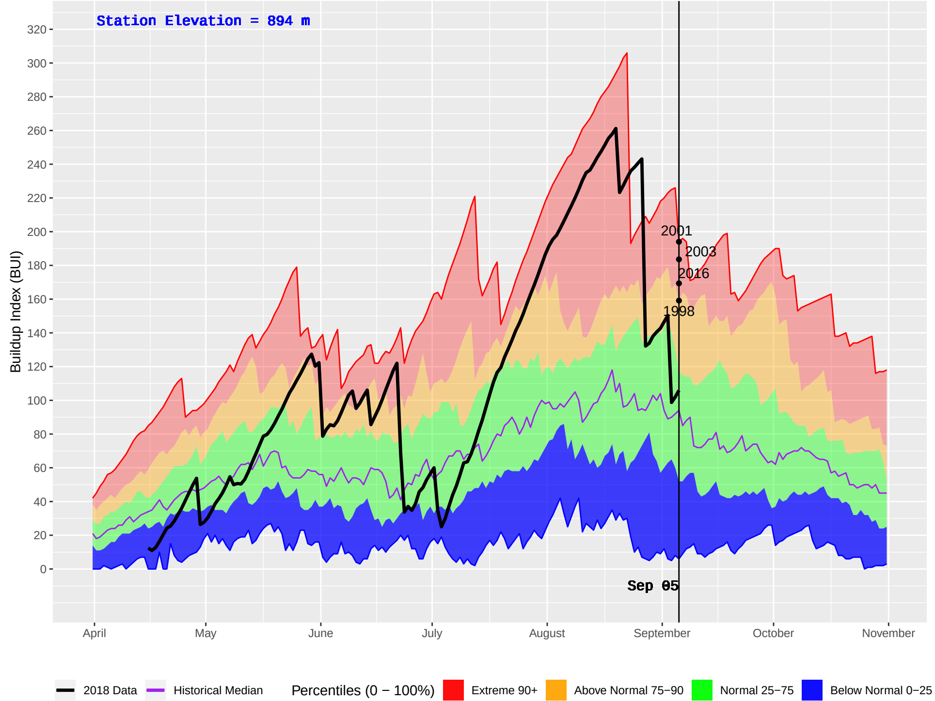
TOBY HUB (417) : Historical (1986–2016) and Current (2018) Daily Buildup Index (BUI)
