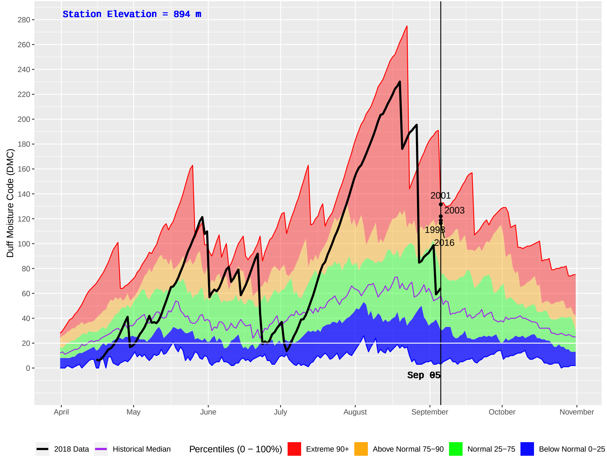
TOBY HUB (417) : Historical (1986–2016) and Current (2018) Daily Duff Moisture Code (DMC)
