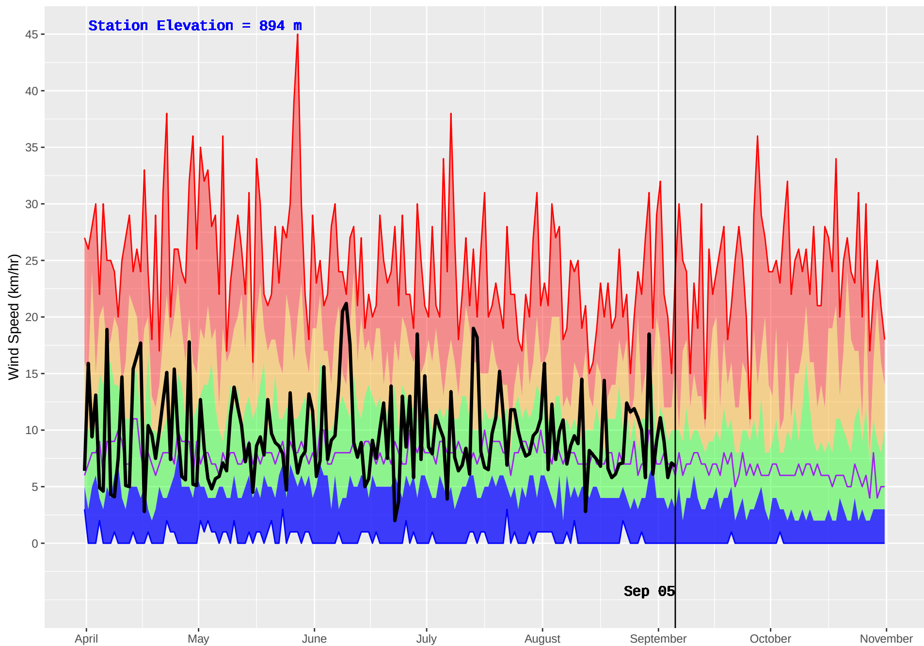
TOBY HUB (417) : Historical (1986–2016) and Current (2018) Daily Wind Speed
