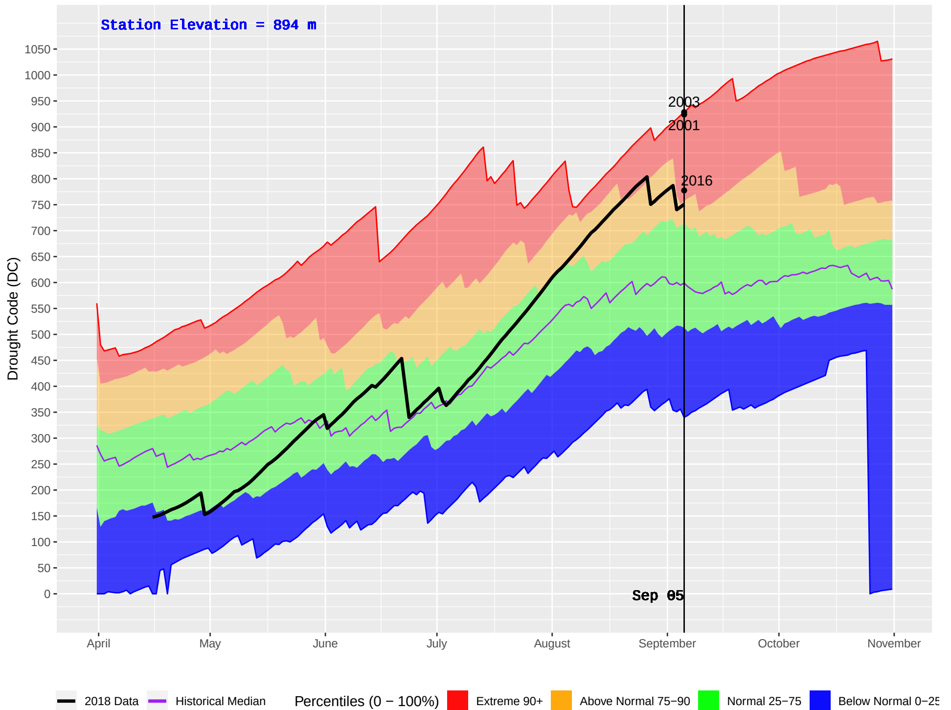
TOBY HUB (417) : Historical (1986–2016) and Current (2018) Daily Drought Code (DC)
