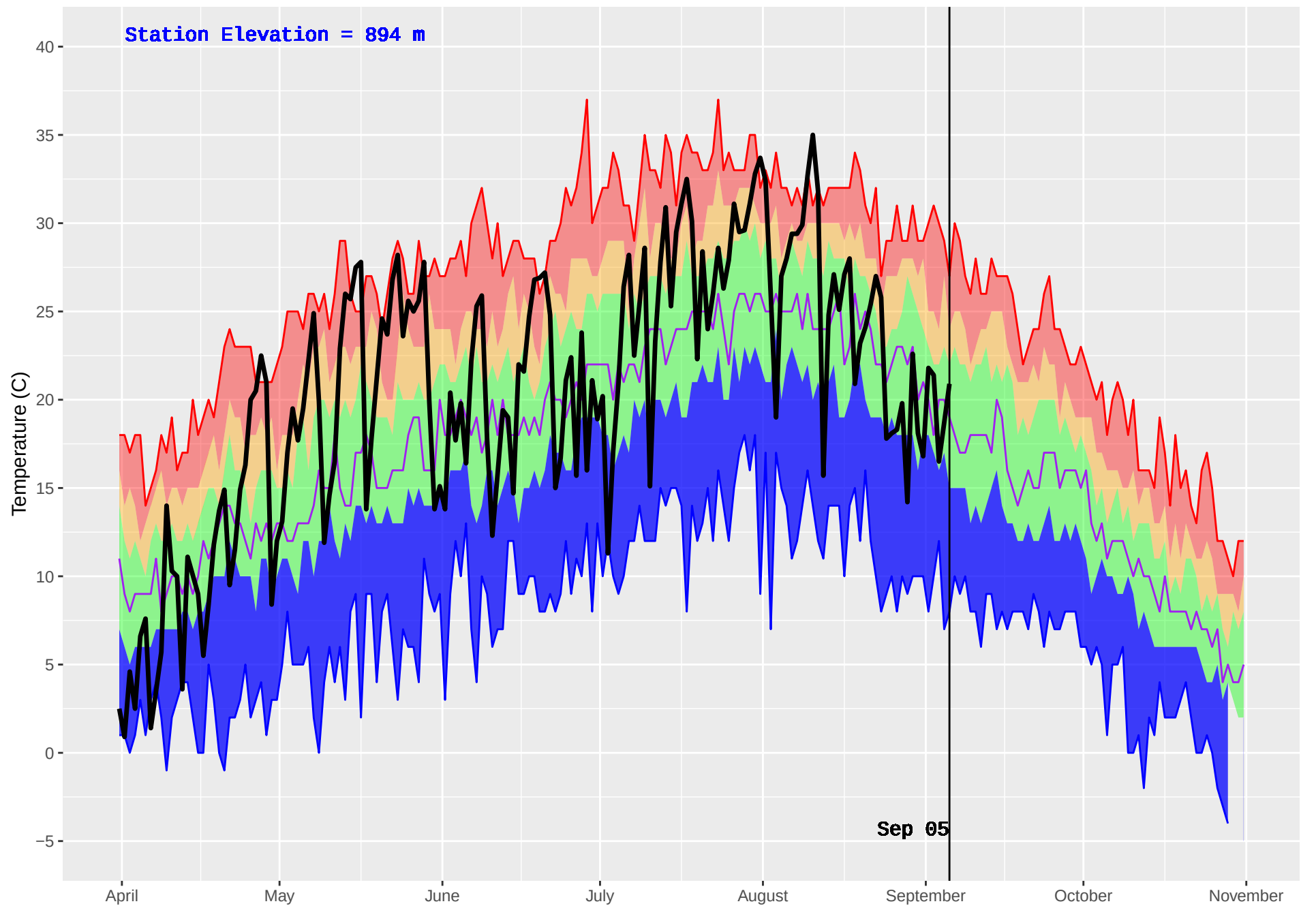
TOBY HUB (417) : Historical (1986–2016) and Current (2018) Daily Temperature
