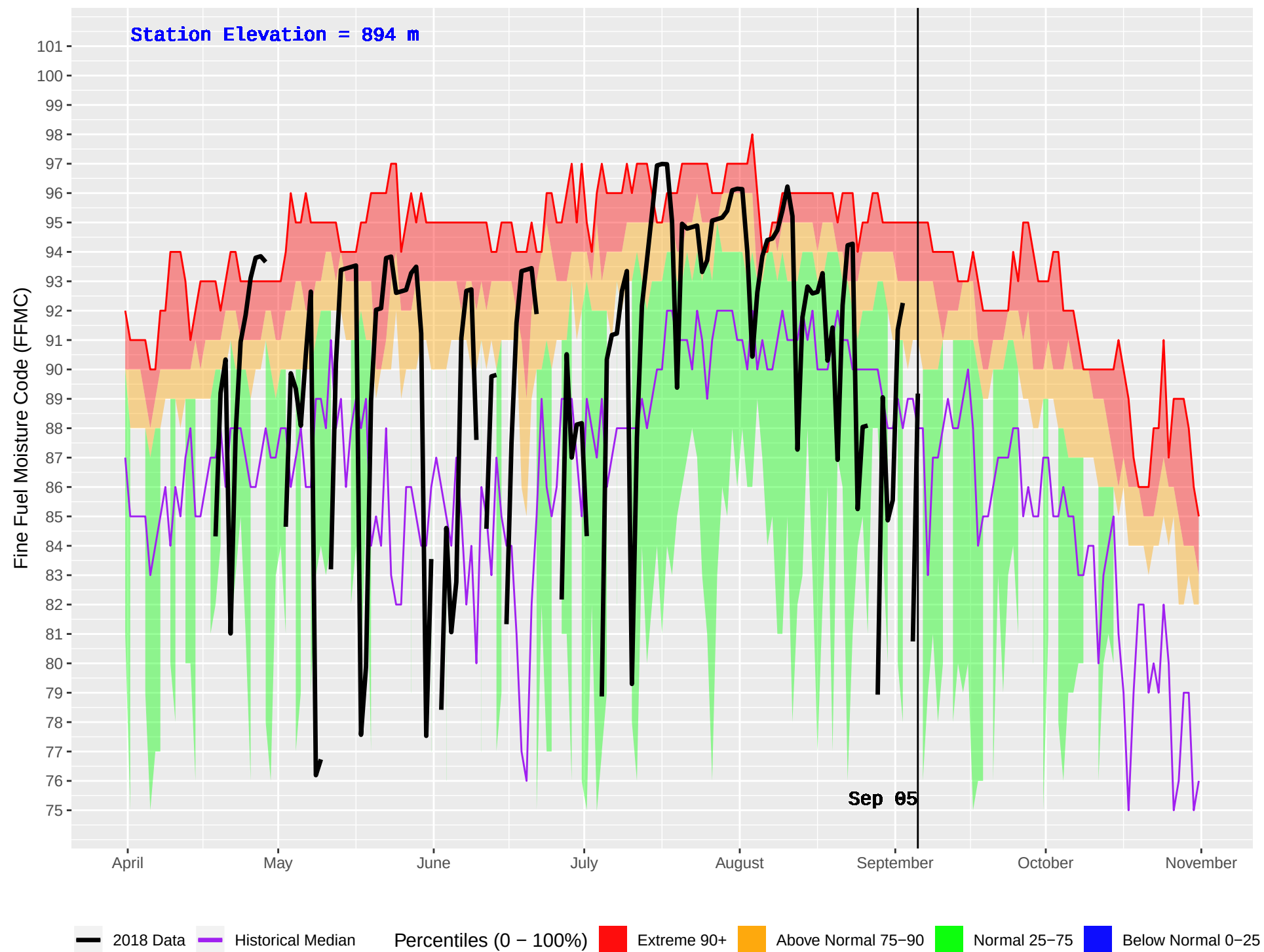
TOBY HUB (417) : Historical (1986–2016) and Current (2018) Daily Fine Fuel Moisture Code (FFMC)
