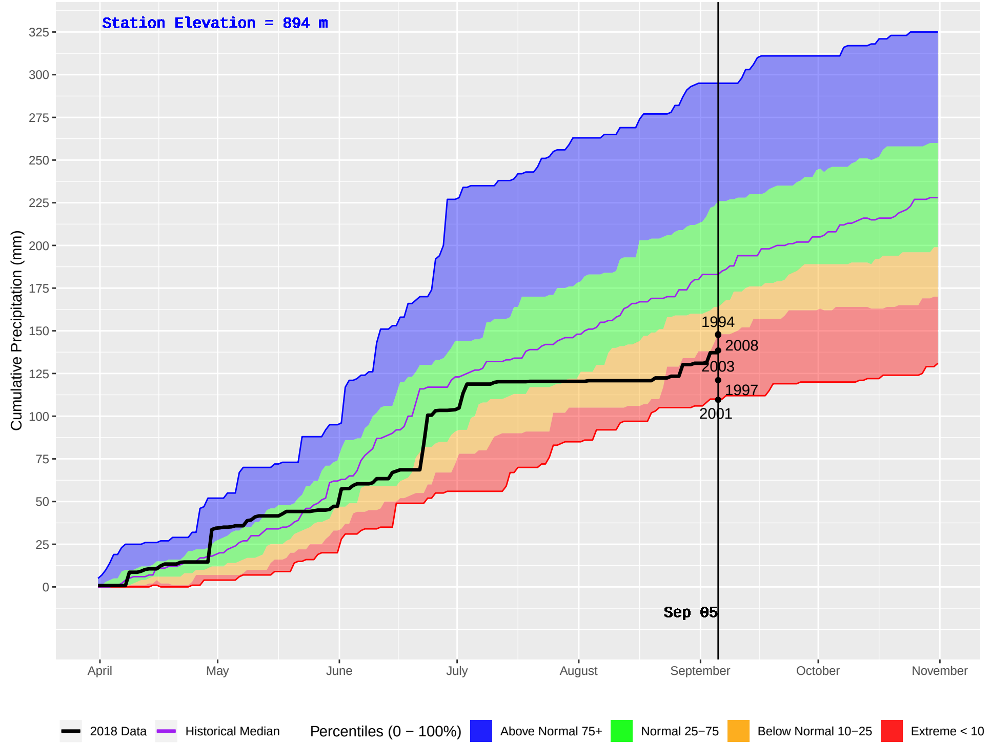
TOBY HUB (417) : Historical (1986–2016) and Current (2018) Daily Cumulative Precipitation
