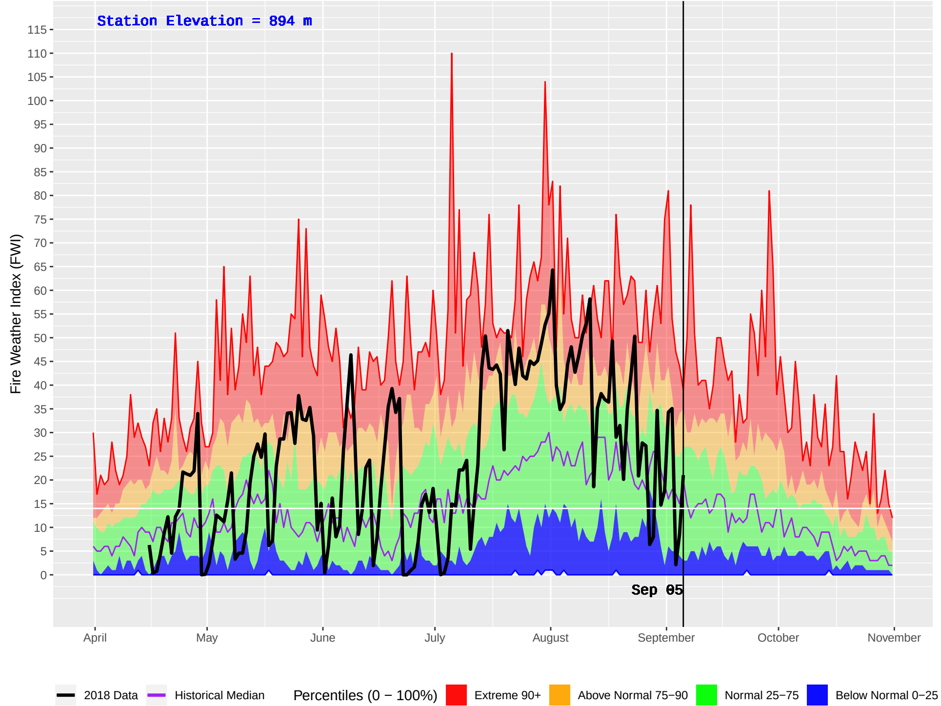
TOBY HUB (417) : Historical (1986–2016) and Current (2018) Daily Fire Weather Index (FWI)
